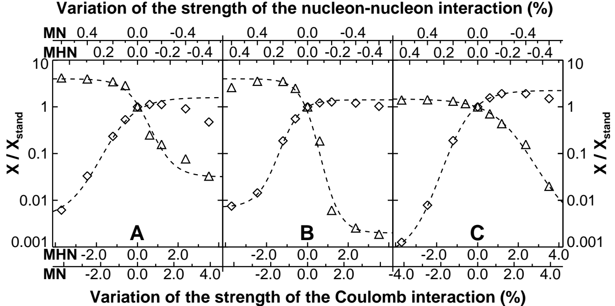
Figure 1: The change of the C and O mass abundances through variations of the strengths of the strong and Coulomb interactions. The C mass abundance, X_C ( \Delta ), and the O mass abundance, X_O ( \diamond ) are shown in (A), (B), and (C) for stars with masses 20 , 5 , and 1.3 M_{\odot} , respectively, in units of the standard values, X_{\text{stand}} . The variations of the strength of the strong and Coulomb interaction are given in the upper and lower scales for the two effective N-N forces MHN and MN. Dashed curves are drawn to show the trends.
