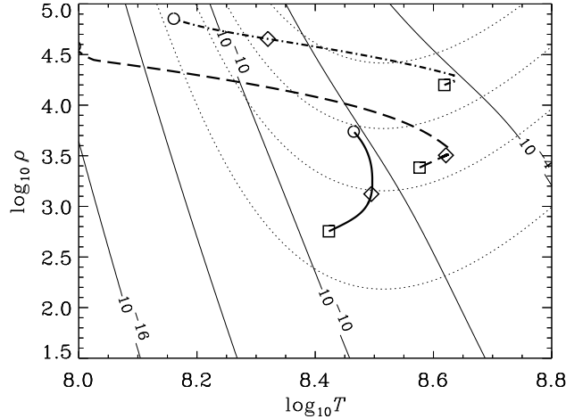
Figure 13. Same as Fig. 7, but the 0_2^+ resonance of ^{12}\text{C} has been increased by 100 keV. The dotted lines mark the positions of f_{\sigma}^{\text{CO}} = 0.95, 0.67, 0.33 and 0.1 (from bottom to top; Eq. (1)). The thick lines show the stratification of the shell with 0.8877 < M_r/M_{\odot} < 0.8887 at \Delta t = 6 yr (dash-dotted), 6.1 yr (dashed) and 15.5 yr (solid line; cf. Fig.6). Equal symbols mark equal mass shells, where \square , \diamond and \circ are located at M_r/M_{\odot} = 0.8877, 0.8882 and 0.8887 , respectively.
